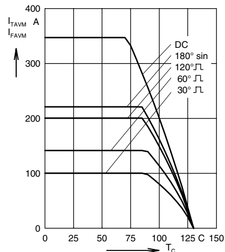
Fig. 6 Maximum forward current at case temperature
