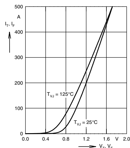
Fig. 3 Forward current versus voltage drop
